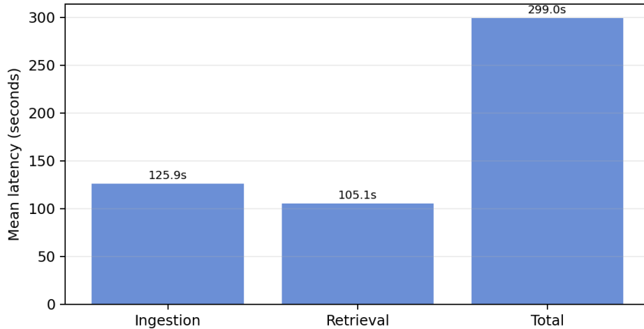
Recall-AI mean processing latency
