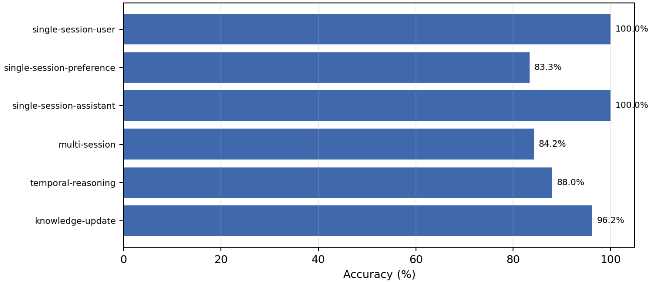
Recall-AI accuracy by LongMemEval_S task category
